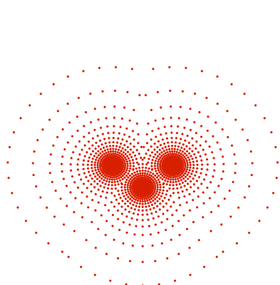
(c) \text{H}_2\text{O}
