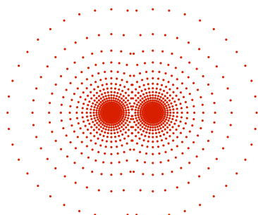
(a) \text{N}_2
