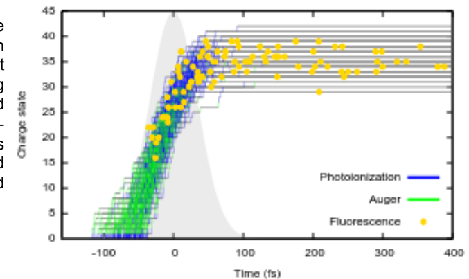
Foto: Exemplary pathways of multiphoton multiple ionization dynamics of Xe at 4.5 keV
