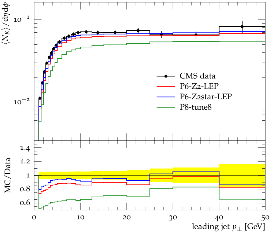
Transverse K_s^0 particle density at \sqrt{s} = 7 TeV, p_{\perp} > 0.6 GeV
