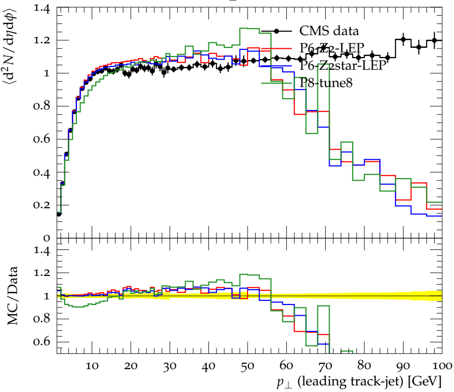
Transverse N_{\text{ch}} density vs. p_{\perp}^{\text{jet } 1} , \sqrt{s} = 7000 GeV
