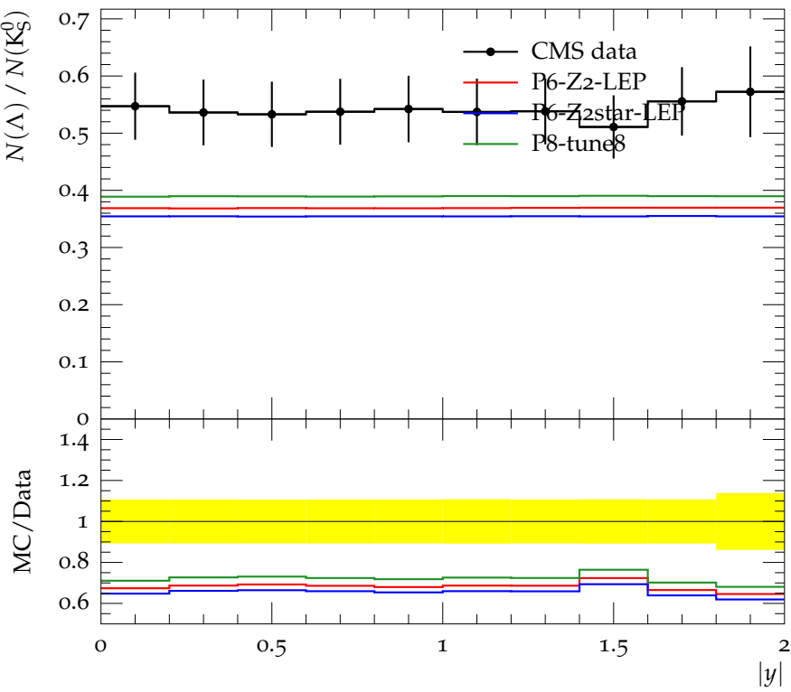
\Lambda/K_S^0 versus rapidity at \sqrt{s} = 7 TeV
