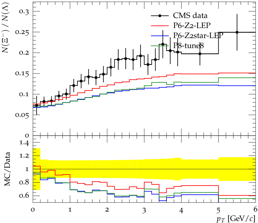
\Xi^- / \Lambda versus transverse momentum at \sqrt{s} = 7 TeV
