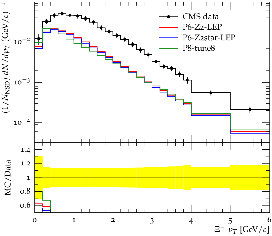
\Xi^- transverse momentum distribution at \sqrt{s} = 7 TeV
