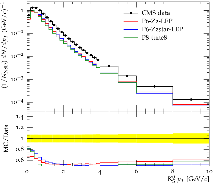
K_S^0 transverse momentum distribution at \sqrt{s} = 7 TeV
