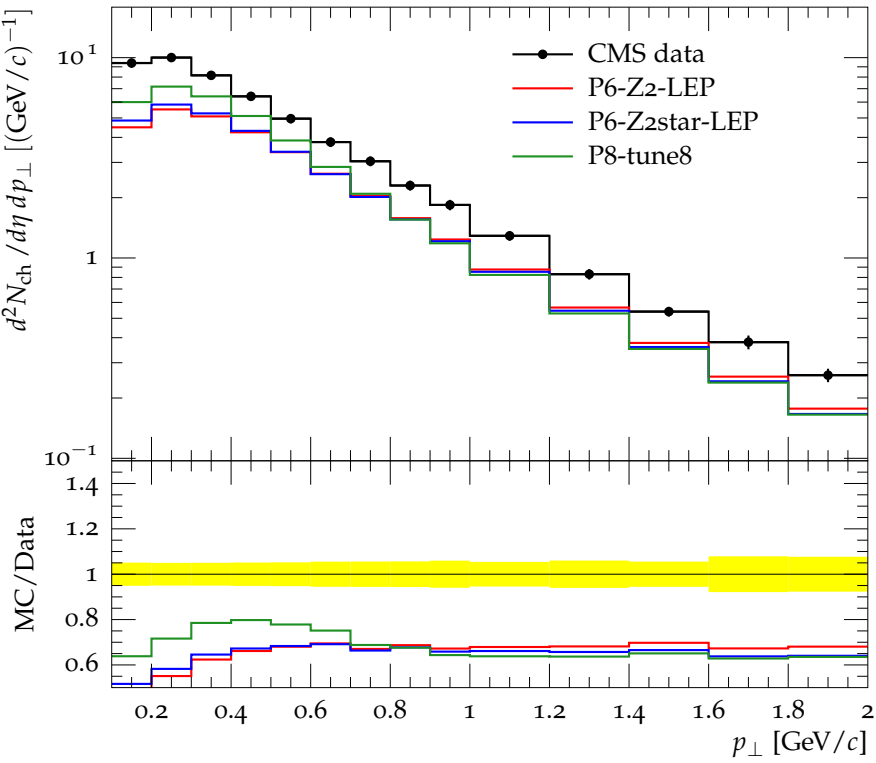
Charged hadron p_{\perp} for |\eta| = 0.9 at \sqrt{s} = 7 TeV
