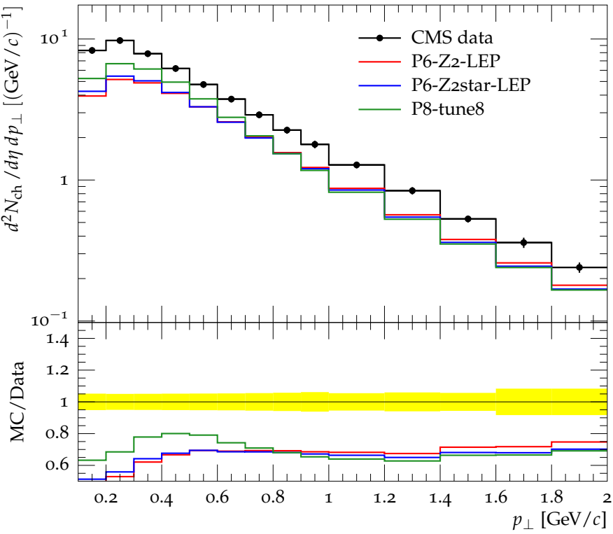
Charged hadron p_{\perp} for |\eta| = 0.1 at \sqrt{s} = 7 TeV
