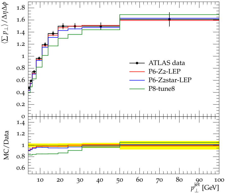
Mean \Sigma p_{\perp} vs. leading jet p_{\perp} , R = 1.0 , Transverse region
