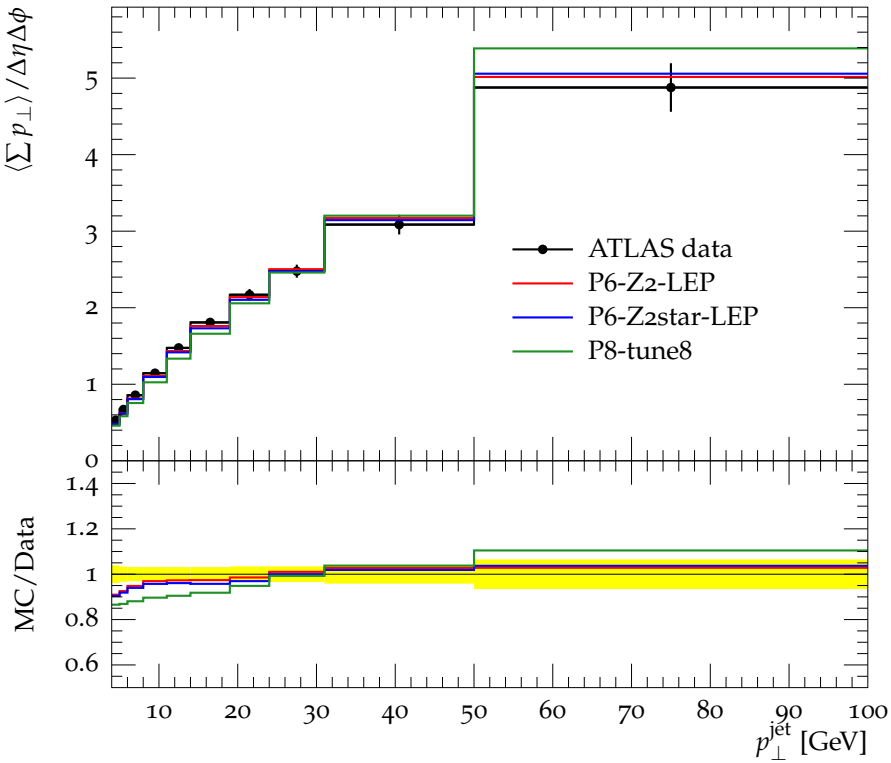
Mean \Sigma p_{\perp} vs. leading jet p_{\perp} , R = 1.0 , Away region
