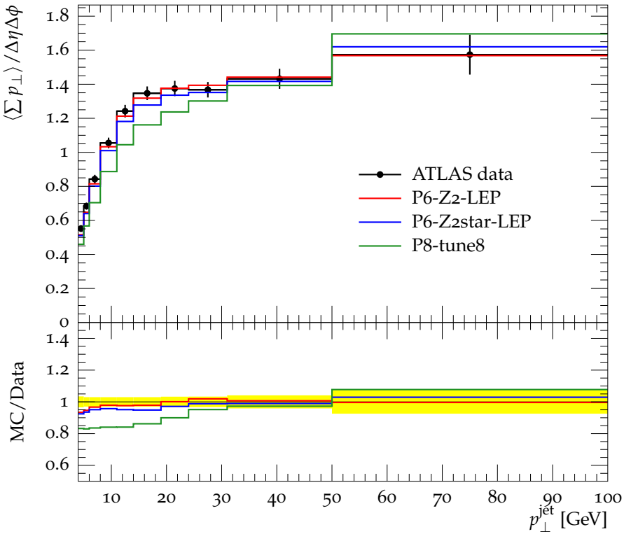
Mean \Sigma p_{\perp} vs. leading jet p_{\perp} , R = 0.8 , Transverse region
