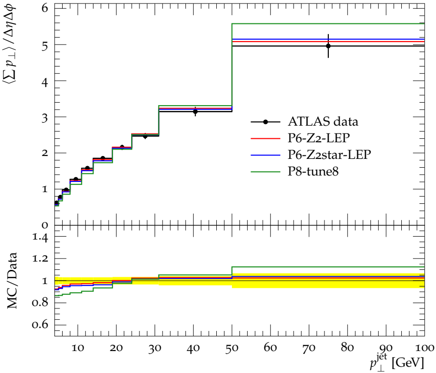
Mean \Sigma p_{\perp} vs. leading jet p_{\perp} , R = 0.8 , Away region
