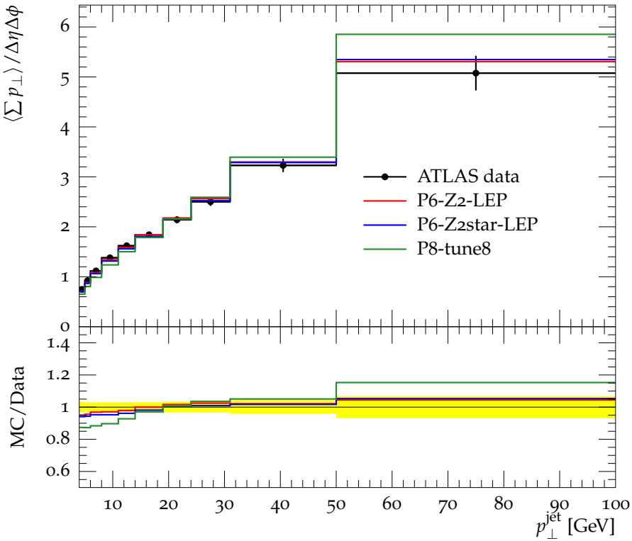
Mean \Sigma p_{\perp} vs. leading jet p_{\perp} , R = 0.6 , Away region
