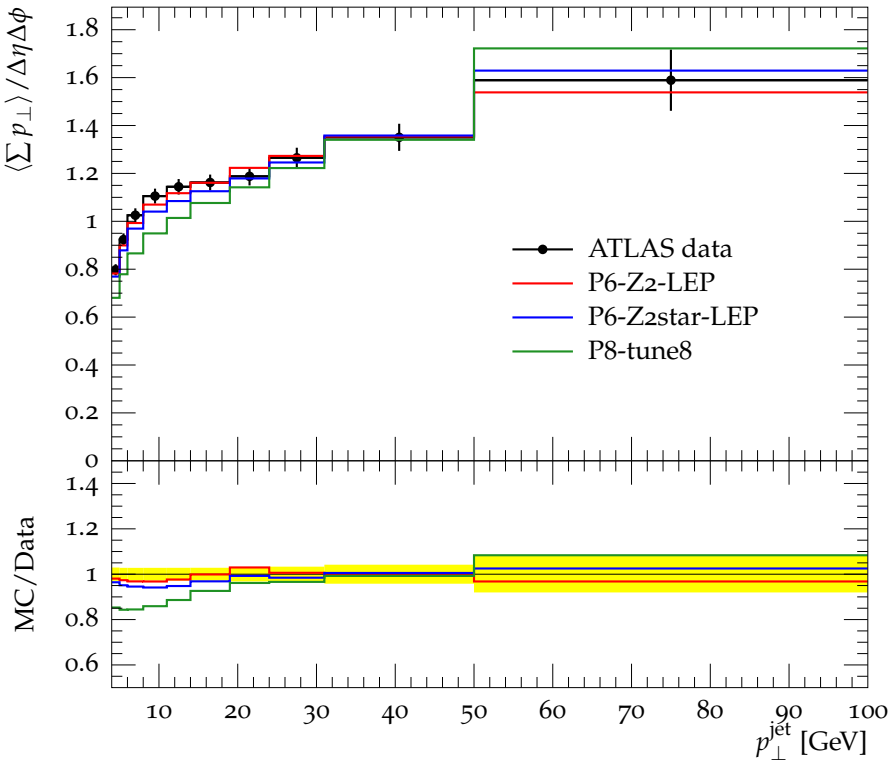
Mean \Sigma p_{\perp} vs. leading jet p_{\perp} , R = 0.4 , Transverse region
