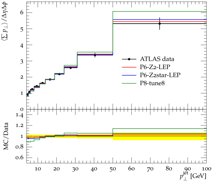
Mean \Sigma p_{\perp} vs. leading jet p_{\perp} , R = 0.4 , Away region
