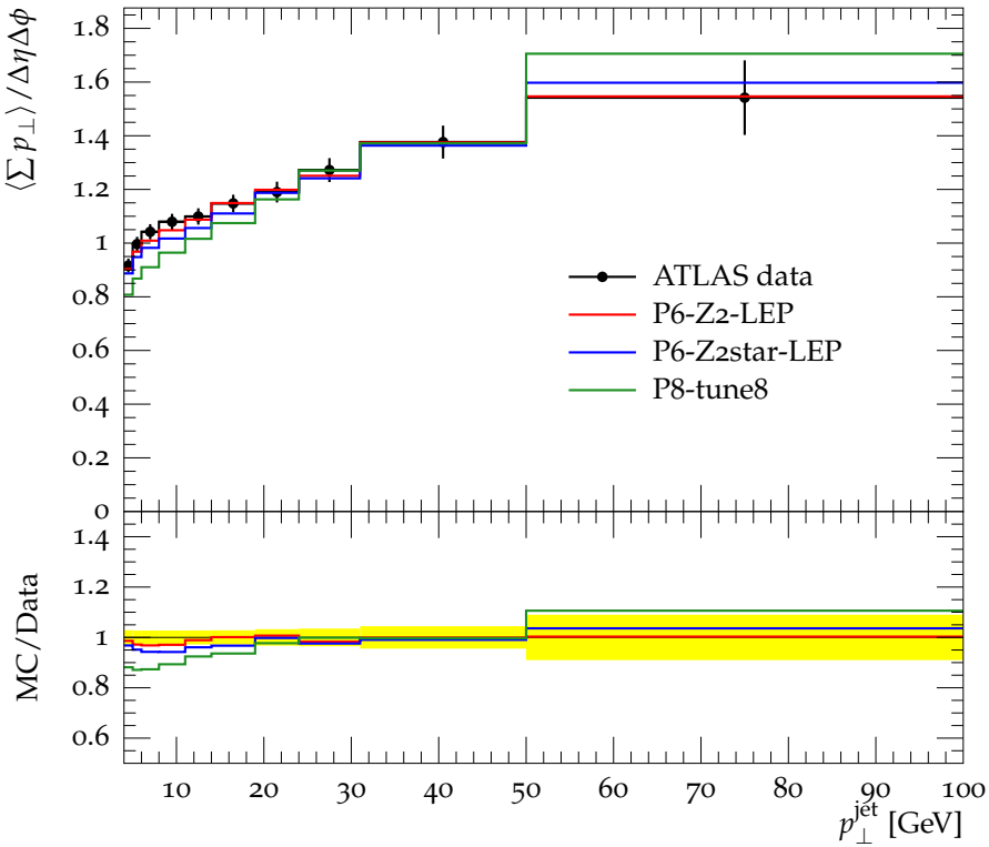
Mean \Sigma p_{\perp} vs. leading jet p_{\perp} , R = 0.2 , Transverse region
