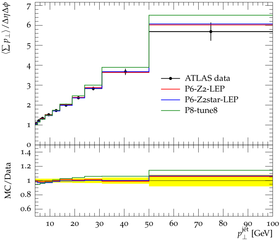
Mean \Sigma p_{\perp} vs. leading jet p_{\perp} , R = 0.2 , Away region
