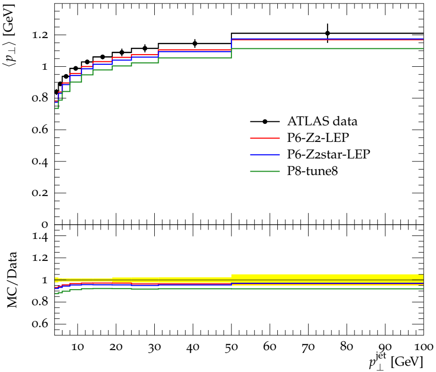
Mean p_{\perp} vs. leading jet p_{\perp} , R = 1.0 , Transverse region
