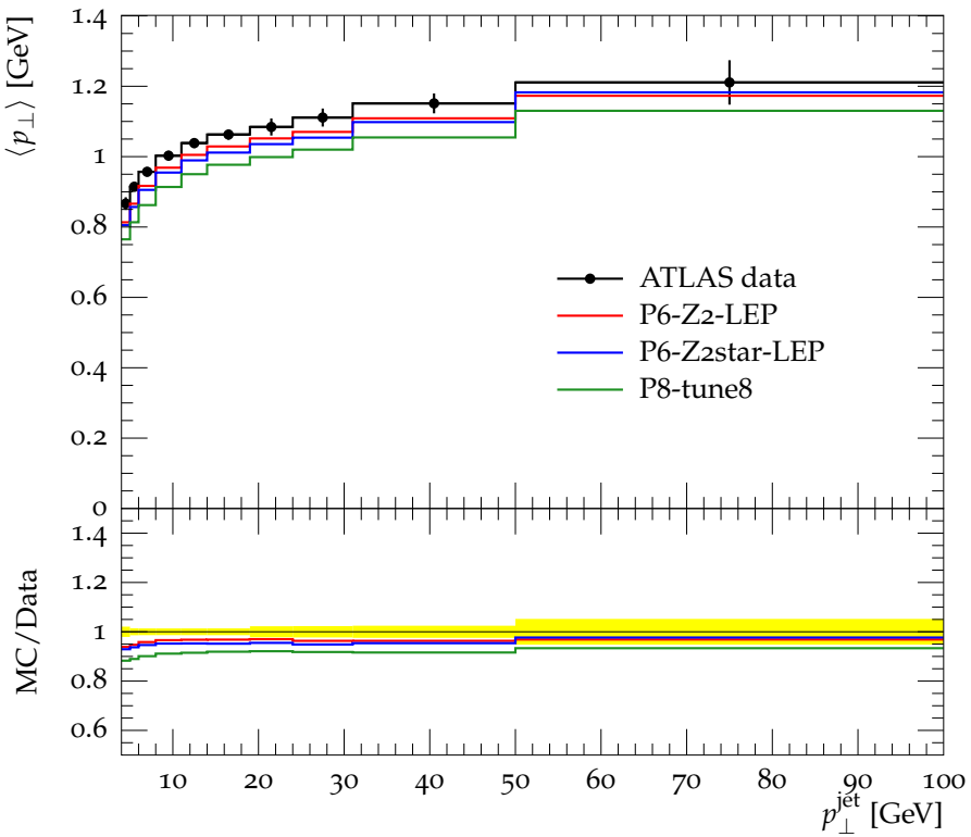
Mean p_{\perp} vs. leading jet p_{\perp} , R = 0.8 , Transverse region
