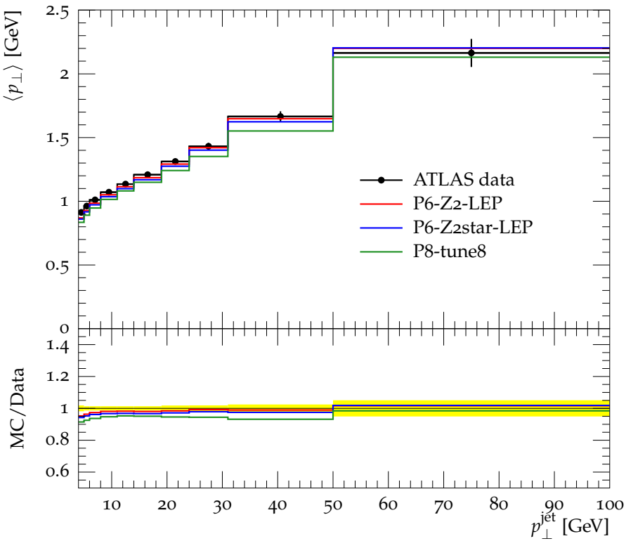
Mean p_{\perp} vs. leading jet p_{\perp} , R = 0.8 , Away region
