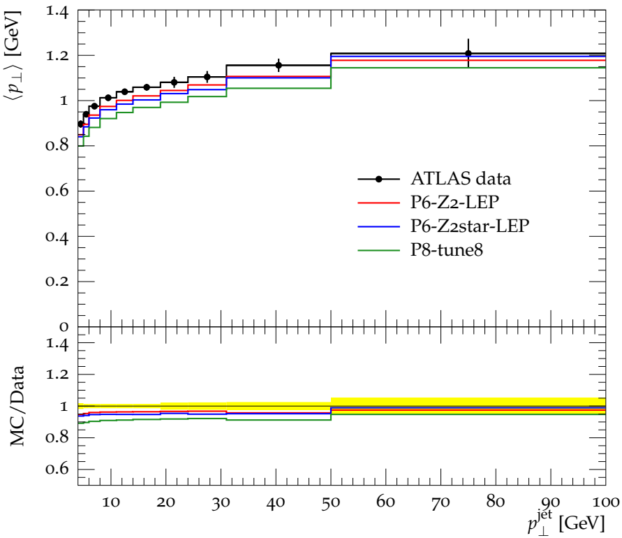
Mean p_{\perp} vs. leading jet p_{\perp} , R = 0.6 , Transverse region
