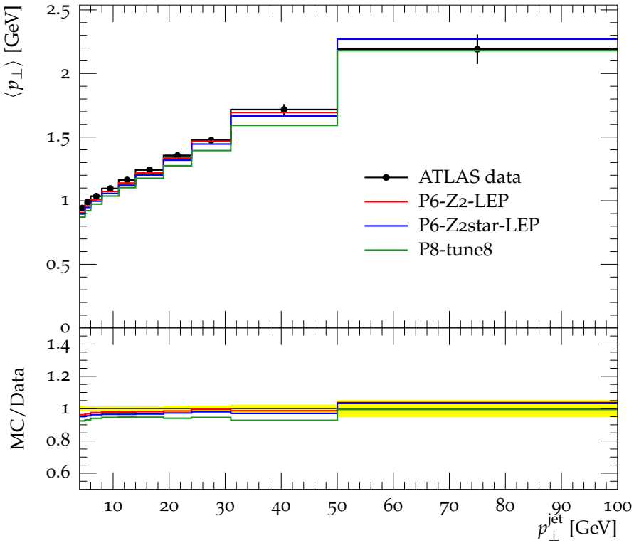
Mean p_\perp vs. leading jet p_\perp , R = 0.6 , Away region
