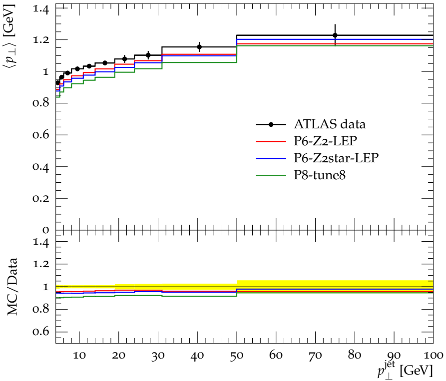
Mean p_{\perp} vs. leading jet p_{\perp} , R = 0.4 , Transverse region
