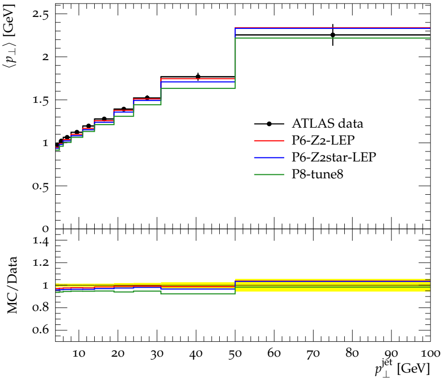
Mean p_{\perp} vs. leading jet p_{\perp} , R = 0.4 , Away region
