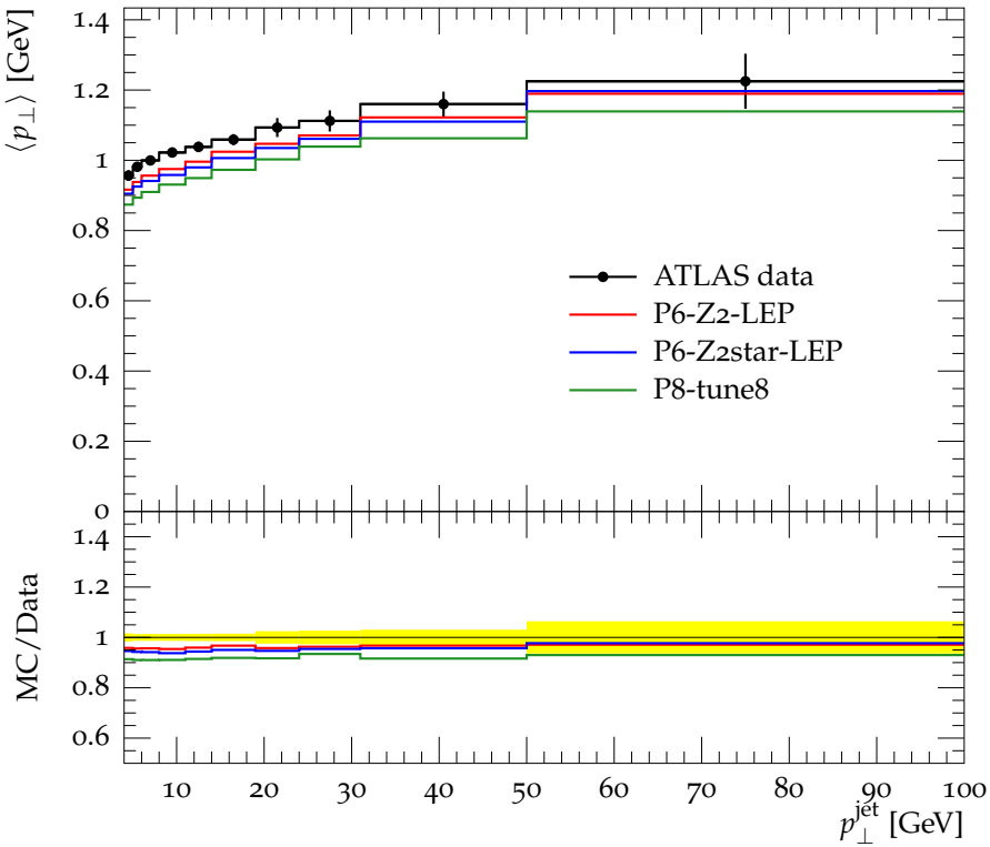
Mean p_{\perp} vs. leading jet p_{\perp} , R = 0.2 , Transverse region
