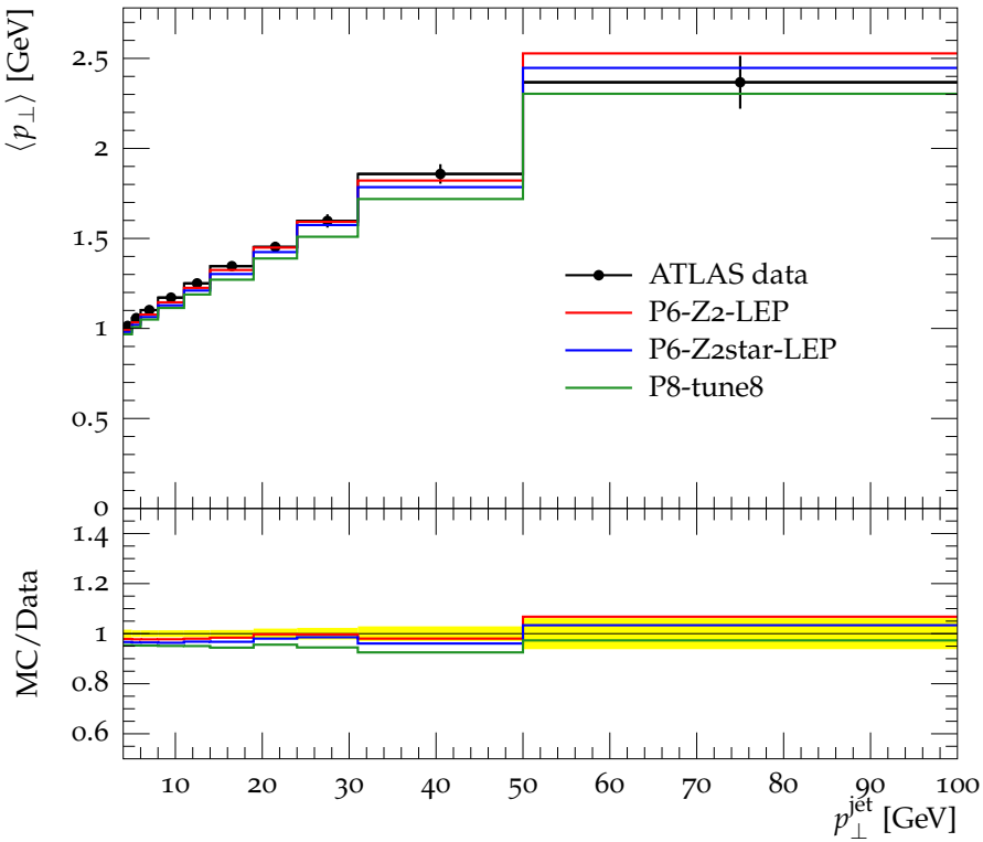
Mean p_{\perp} vs. leading jet p_{\perp} , R = 0.2 , Away region
