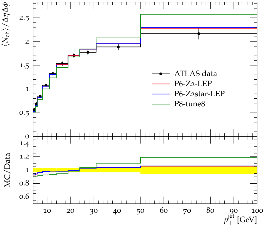
Mean N_{\text{ch}} vs. leading jet p_{\perp} , R = 1.0 , Away region
