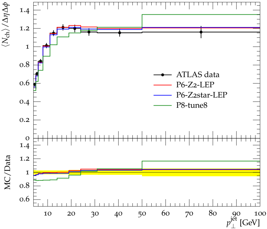
Mean N_{\text{ch}} vs. leading jet p_{\perp} , R = 0.8 , Transverse region
