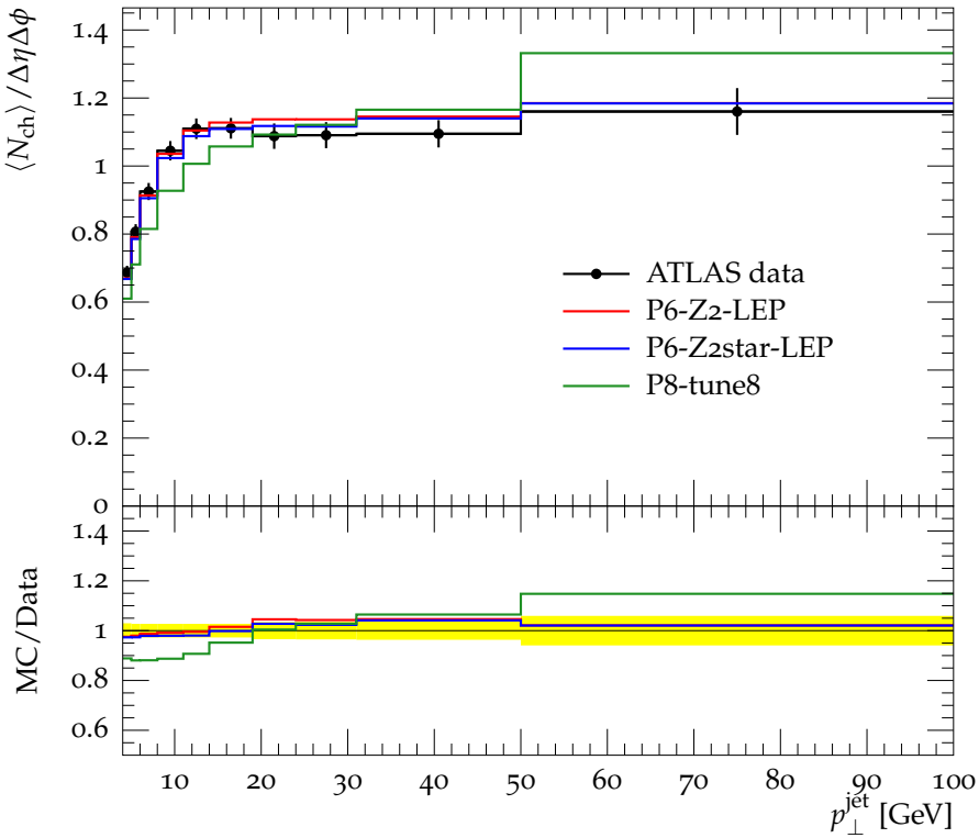
Mean N_{\text{ch}} vs. leading jet p_{\perp} , R = 0.6 , Transverse region
