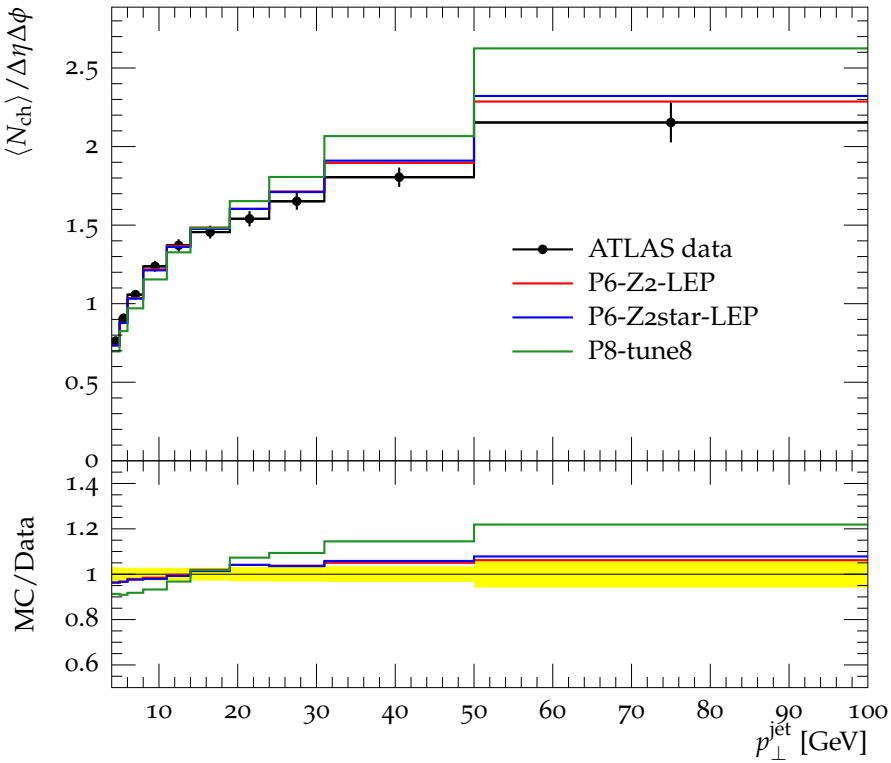
Mean N_{\text{ch}} vs. leading jet p_{\perp} , R = 0.6 , Away region
