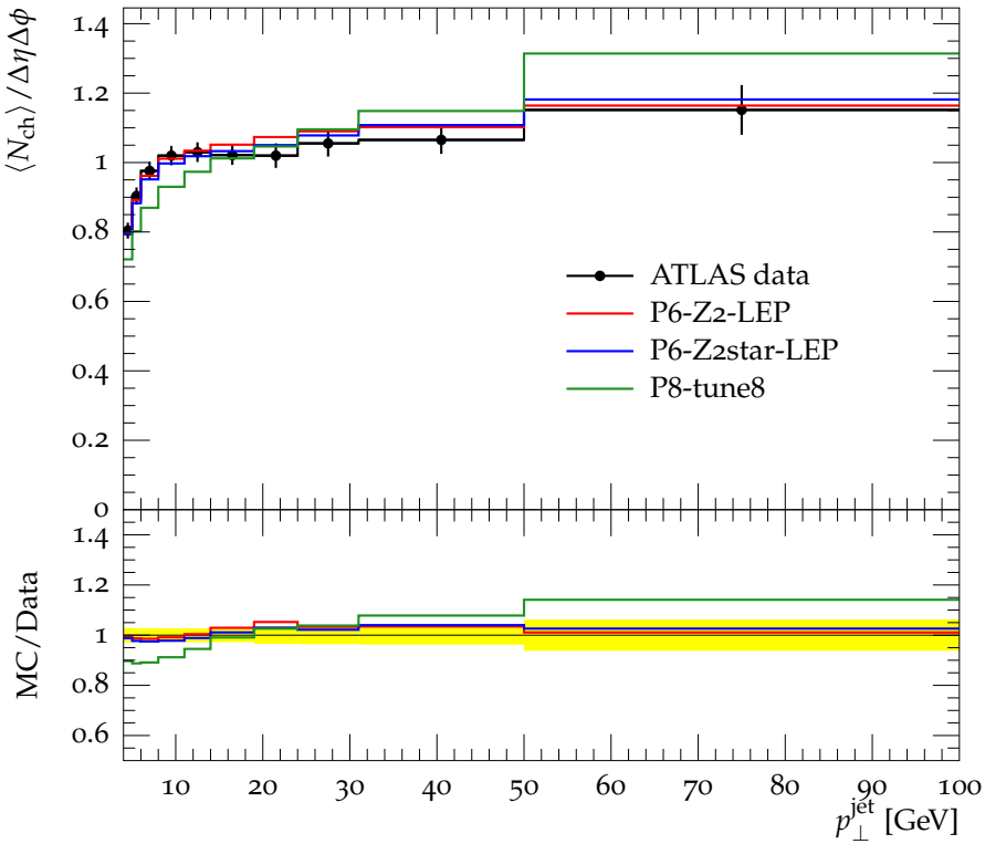
Mean N_{\text{ch}} vs. leading jet p_{\perp} , R = 0.4 , Transverse region
