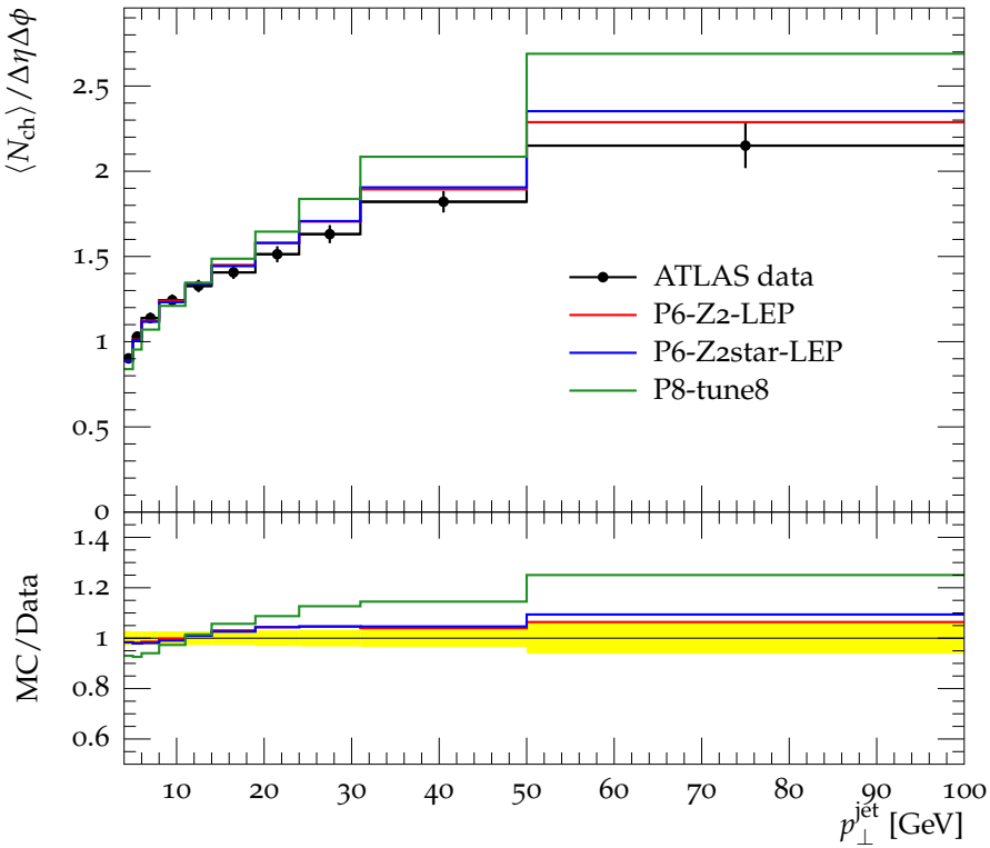
Mean N_{\text{ch}} vs. leading jet p_{\perp} , R = 0.4 , Away region
