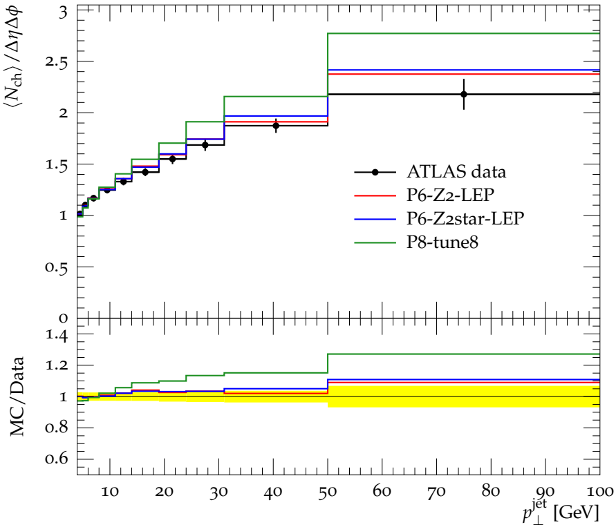
Mean N_{\text{ch}} vs. leading jet p_{\perp} , R = 0.2 , Away region
