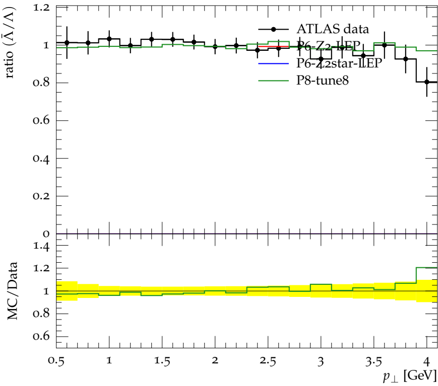
Production ratio of \bar{\Lambda} and \Lambda vs. p_{\perp} , \sqrt{s} = 7000 GeV
