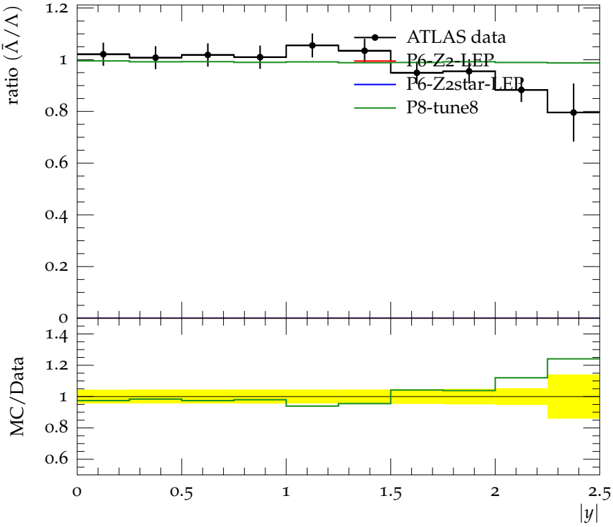
Production ratio of \bar{\Lambda} and \Lambda vs. |y| , \sqrt{s} = 7000 GeV
