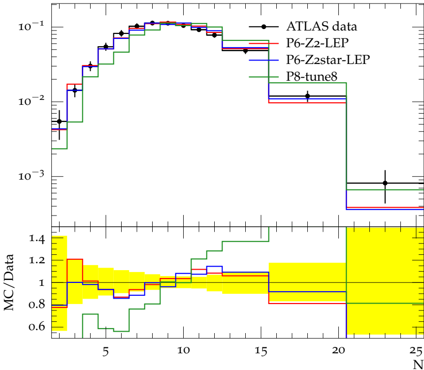
Charged jet multiplicity (anti- k_t , R = 0.6 , y 1.5-1.9, p_\perp 24.0-40.0)
