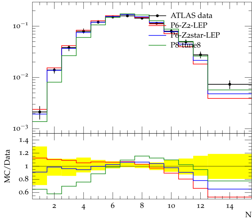
Charged jet multiplicity (anti- k_t , R = 0.6 , y 1.5-1.9, p_\perp 10.0-15.0)
