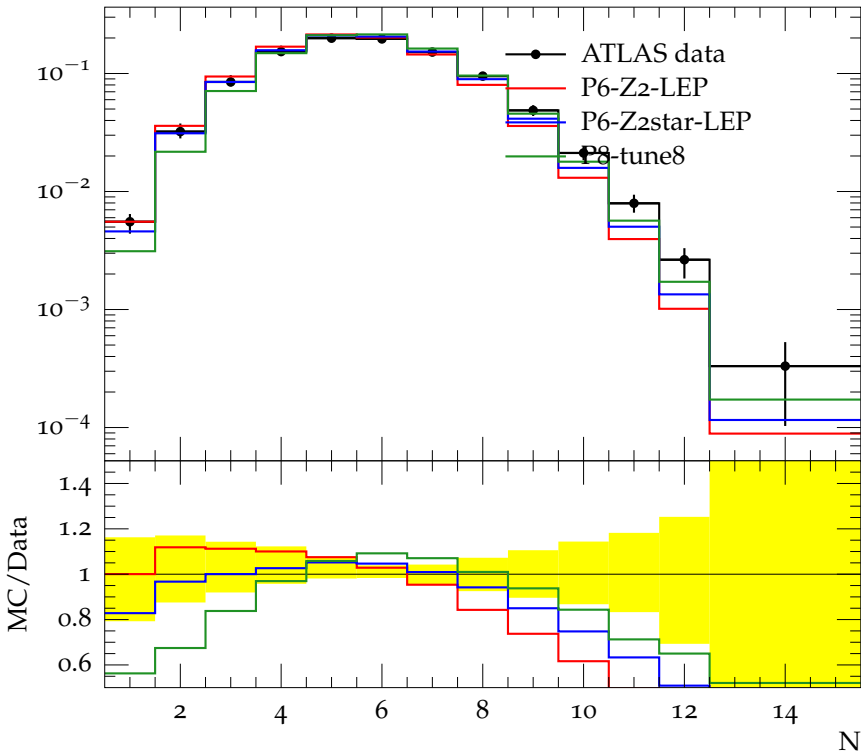
Charged jet multiplicity (anti- k_t , R = 0.6 , y 1.5-1.9, p_\perp 6.0-10.0)
