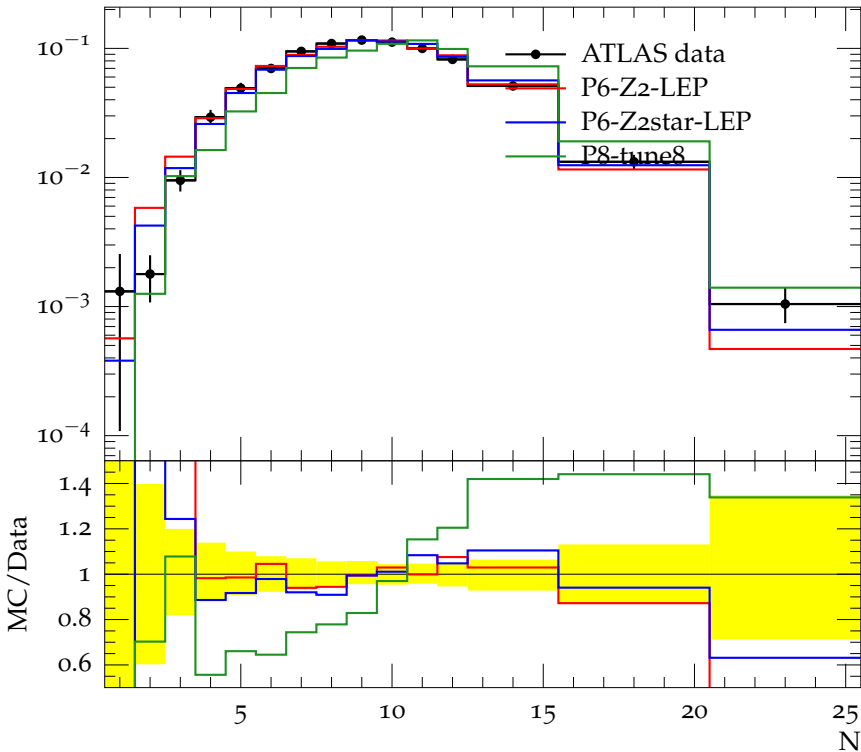
Charged jet multiplicity (anti- k_t , R = 0.6 , y 1.0-1.5, p_\perp 24.0-40.0)
