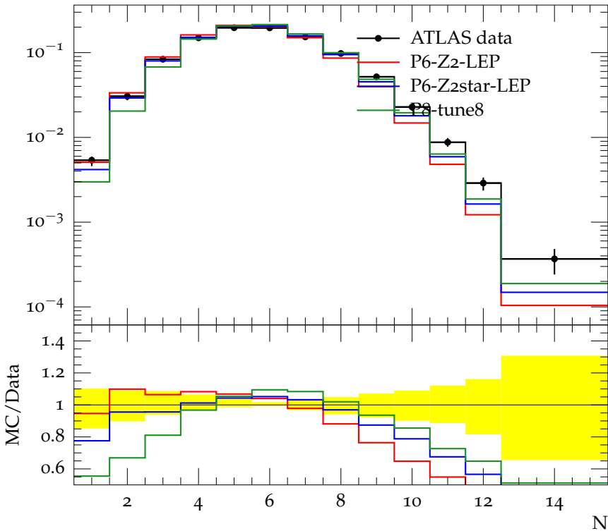
Charged jet multiplicity (anti- k_t , R = 0.6 , y 1.0-1.5, p_\perp 6.0-10.0)
