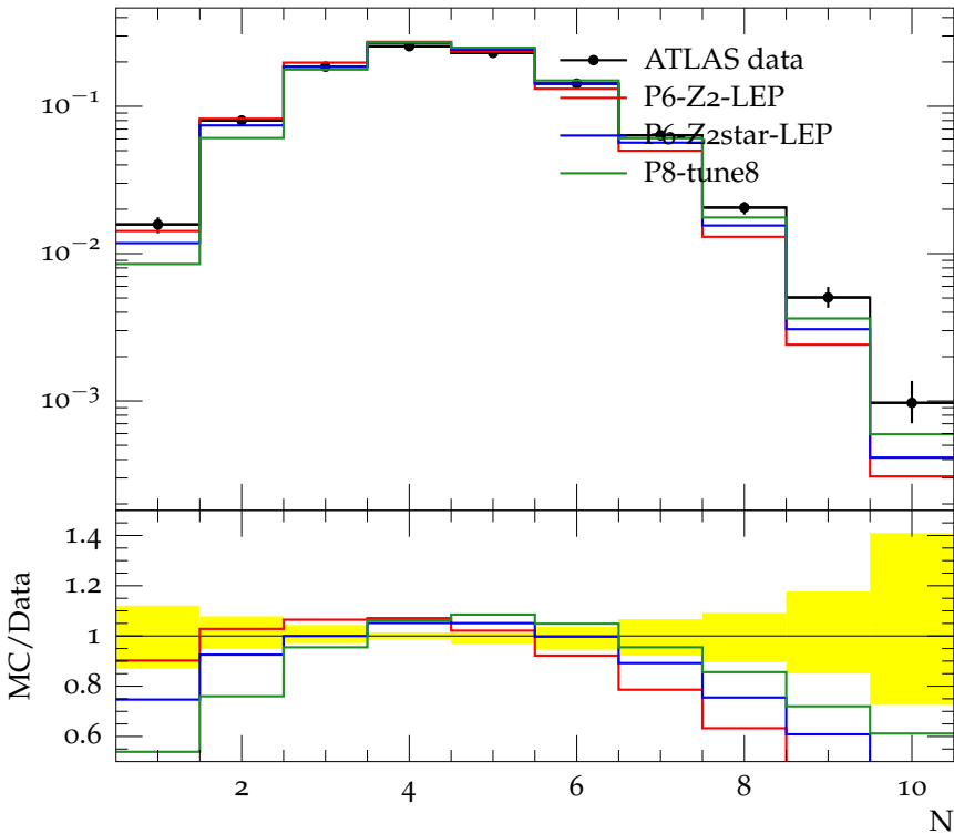
Charged jet multiplicity (anti- k_t , R = 0.6 , y 1.0-1.5, p_\perp 4.0-6.0)
