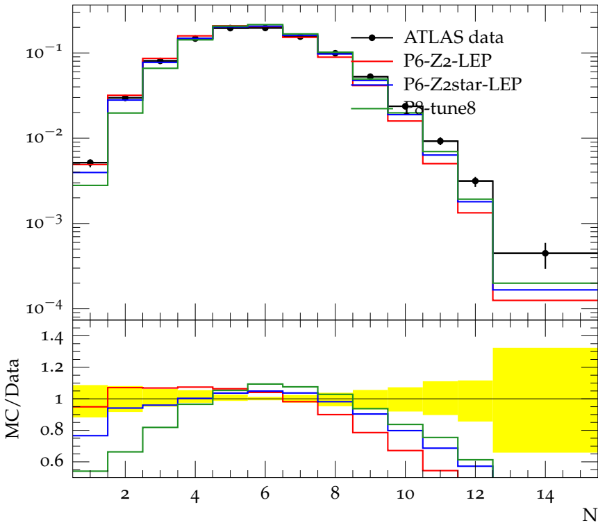
Charged jet multiplicity (anti- k_t , R = 0.6 , y 0.5-1.0, p_\perp 6.0-10.0)
