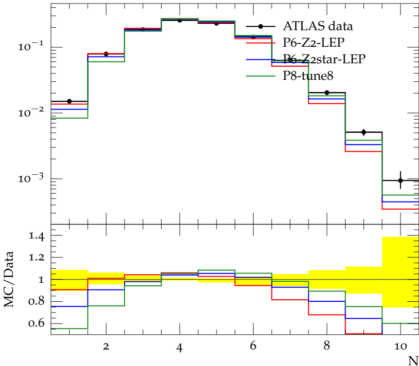
Charged jet multiplicity (anti- k_t , R = 0.6 , y 0.5-1.0, p_\perp 4.0-6.0)
