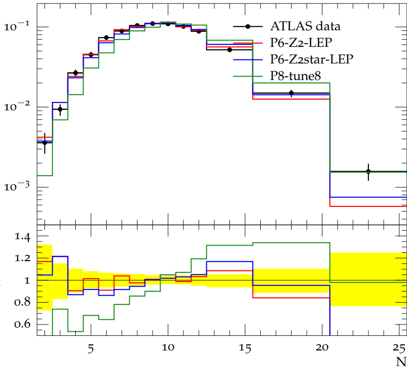
Charged jet multiplicity (anti- k_t , R = 0.6 , y 0.0-0.5, p_\perp 24.0-40.0)
