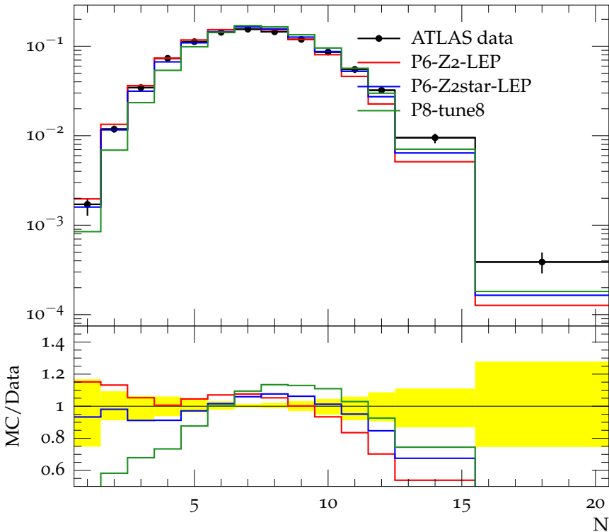
Charged jet multiplicity (anti- k_t , R = 0.6 , y 0.0-0.5, p_\perp 10.0-15.0)
