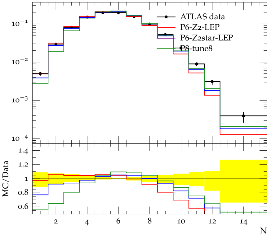
Charged jet multiplicity (anti- k_t , R = 0.6 , y 0.0-0.5, p_\perp 6.0-10.0)
