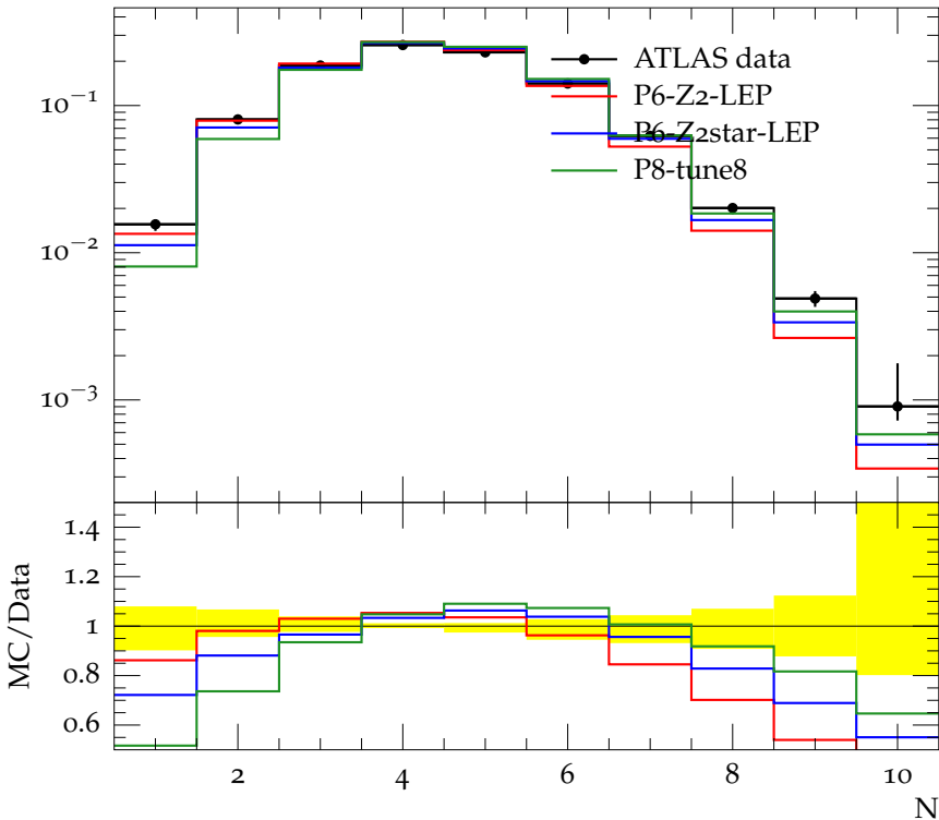
Charged jet multiplicity (anti- k_t , R = 0.6 , y 0.0-0.5, p_\perp 4.0-6.0)
