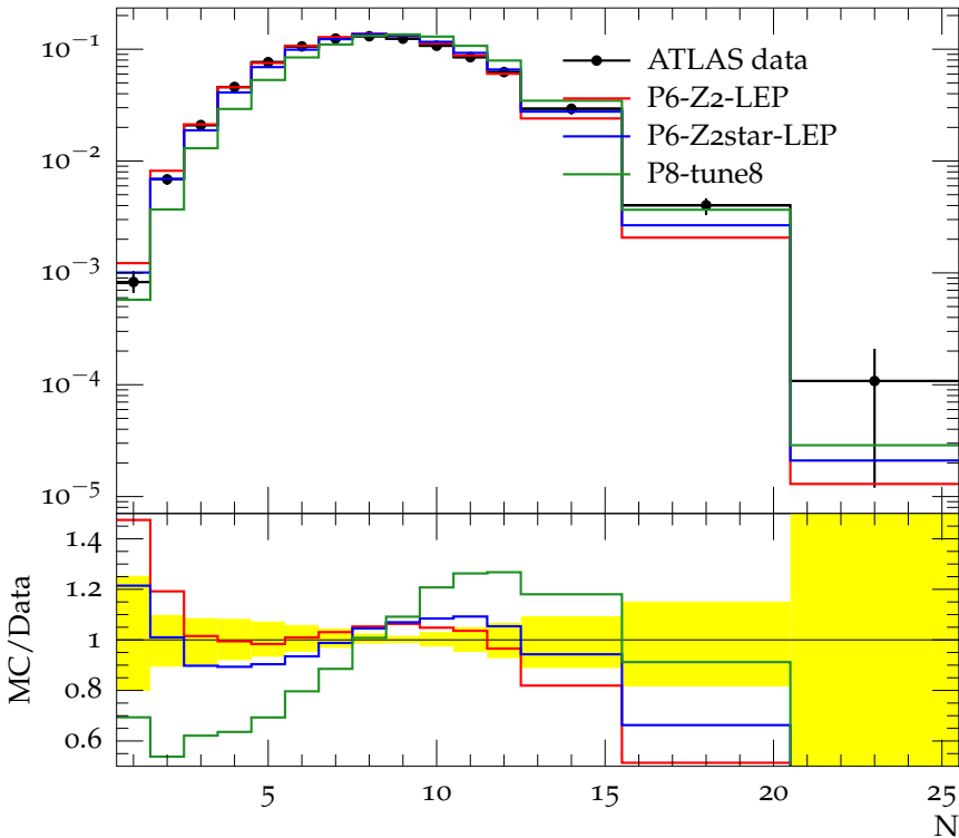
Charged jet multiplicity (anti- k_t , R = 0.6 , y 0.0-1.9, p_\perp 15.0-24.0)
